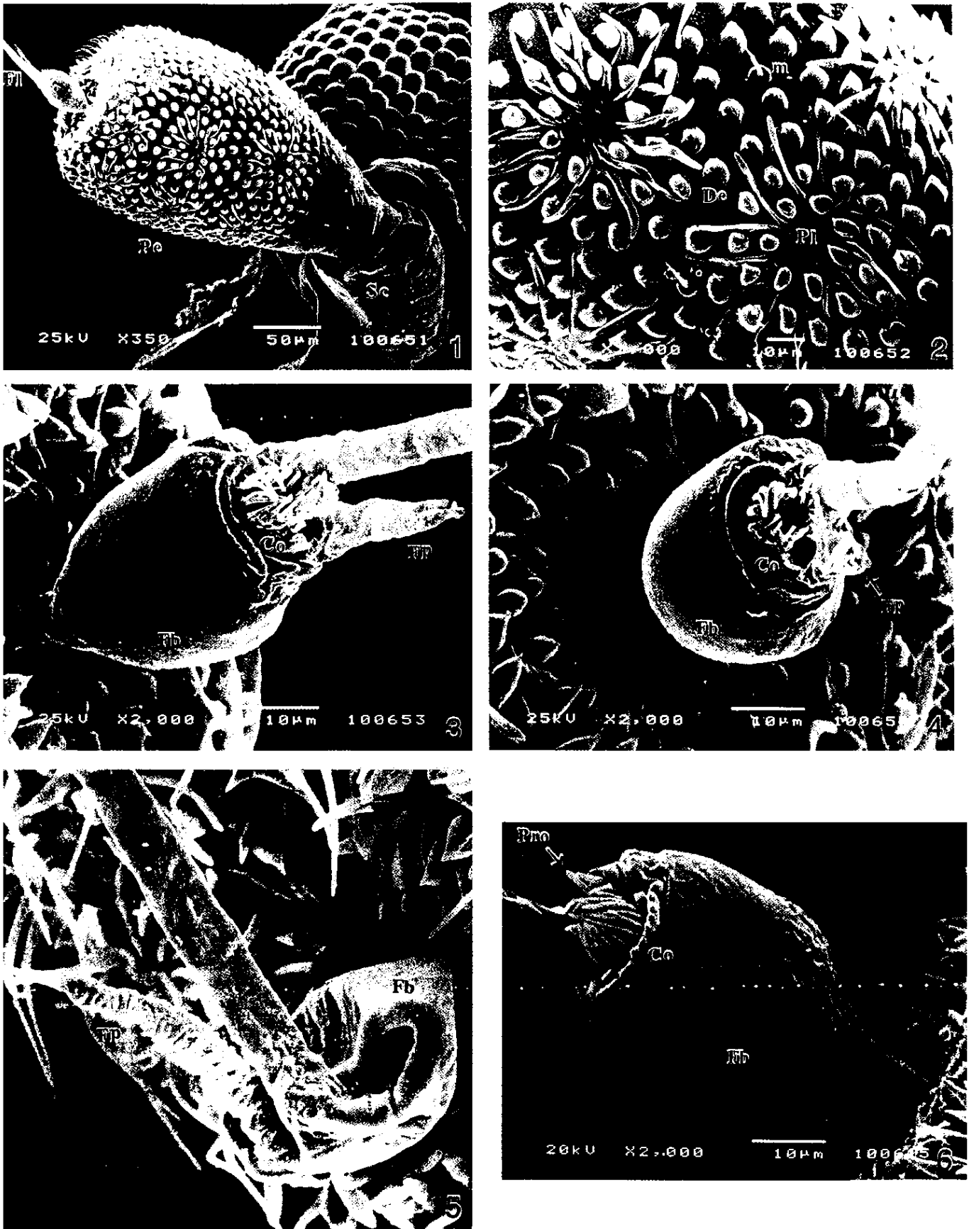
Figs. 1-6. Scanning electron micrographs of antennal sensilla of planthoppers. 1-4. Achilixius sandakanensis Muir (Achilixiidae): 1. antenna, showing the scape (Sc), pedicel (Pe) and flagellum (Fl); 2. surface of pedicel, showing microtrichia (m), cuticular denticles (De), and plaque organs (Pl); 3. swollen, amphora-like, flagellar base (Fb), showing coeloconic sensillum (Co) and basal flagellar process (Fp) with digitate tip; 4. same. 5. Betacixius nigromarginalis Fennah (Cixiidae), swollen, amphora-like, flagellar base (Fb), showing basal flagellar process (Fp) with digitate tip. 6. Proutista sp. (Derbidae), swollen flagellar base (Fb), showing tufts of hairs surrounding the opening of the coeloconic sensillum (Co) and the 'three short conical protuberances (Pro)'.
