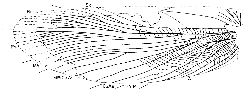
Fig. 1. Nipponohagla kaga sp. nov., forewing. \times 2.2 Holotype, NSM-PA12002. Kuwajima, Lower Cretaceous.
