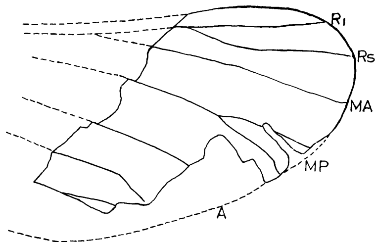
Fig. 3. Fulgoridium? matsuoi sp. nov., hind wing. \times 8 Holotype, NSM-PA12005. Kuwajima, Lower Cretaceous.
