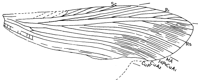
Fig. 2. Nipponohagla kaga sp. nov., hind wing. \times 2.2 Holotype, NSM-PA12003. Kuwajima, Lower Cretaceous.
