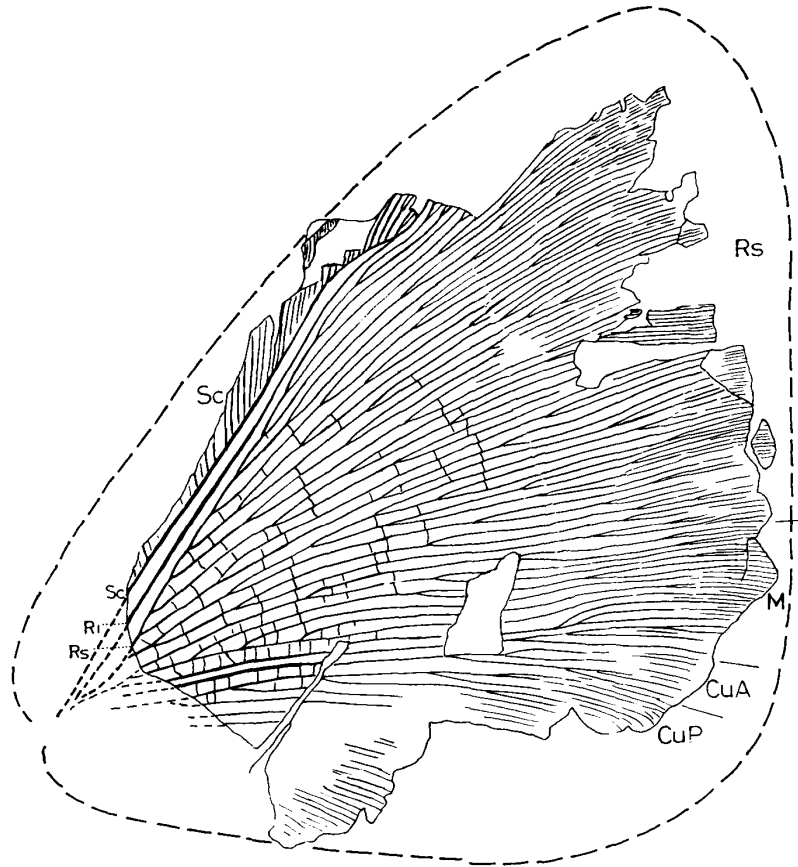
Fig. 6. Kagapsychoptera aranea sp. nov., forewing. \times 2.2 Holotype, NSM-PA12004. Kuwajima, Lower Cretaceous.
