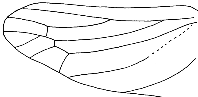
Fig. 5. Scytinoptera kaltanica BECKER-MIGDISOVA, hind wing. Kuznetzk Basin, Permian. (After BECKER-MIGDISOVA, 1961 & 1962.)
